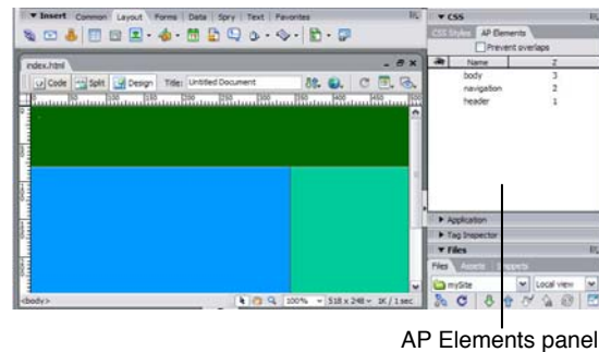
Figure 7 Multiple divs on page
